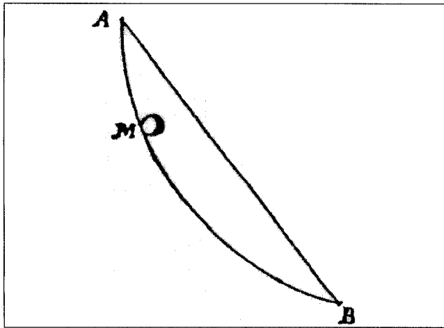
Fig. 2. The Brachystochrone Problem ( Acta Eruditorum , June 1696, p. 269).
