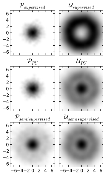
Figure 4.2: Empirical densities of the synthetic data used for training per problem setting (visualized in input space). The supervised densities (top row) are based on samples of the underlying positive and negative classes. The use of high contamination (30%) induces similar empirical densities for \mathcal{P} and \mathcal{U} in the semi-supervised setting (bottom row).
