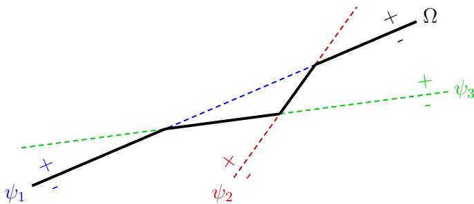
Figure 4.3: The effect of majority voting in an ensemble \Omega with three linear base models ( \psi_1 , \psi_2 , \psi_3 ). The thick black line represents the overall decision boundary of \Omega . The use of majority voting generally induces nonlinear decision boundaries, e.g., when using linear base models the ensemble has a piecewise linear decision boundary.
