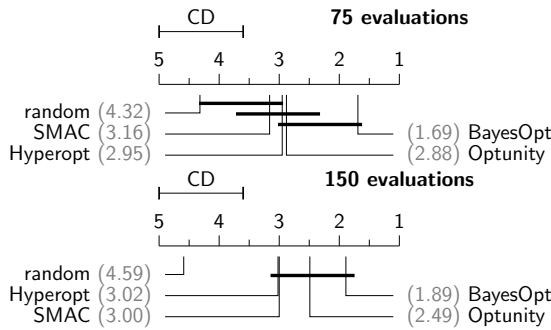
Figure 6.1: Critical difference diagrams for 75 and 150 evaluations to tune an SVM with RBF kernel, depicting average rank per optimizer (lower is better). Optimizers without statistically significant performance differences at \alpha = 5\% are linked.
