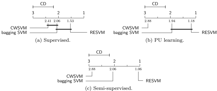
Figure 4.2: Critical difference diagrams for each setting. Groups of algorithms that are not significantly different at the 5% significance level are connected.
